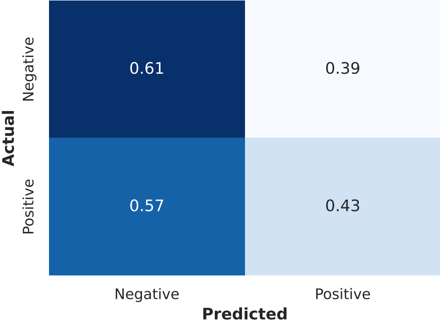
Confusion Matrix - Model 3 - Test (Test Split)
