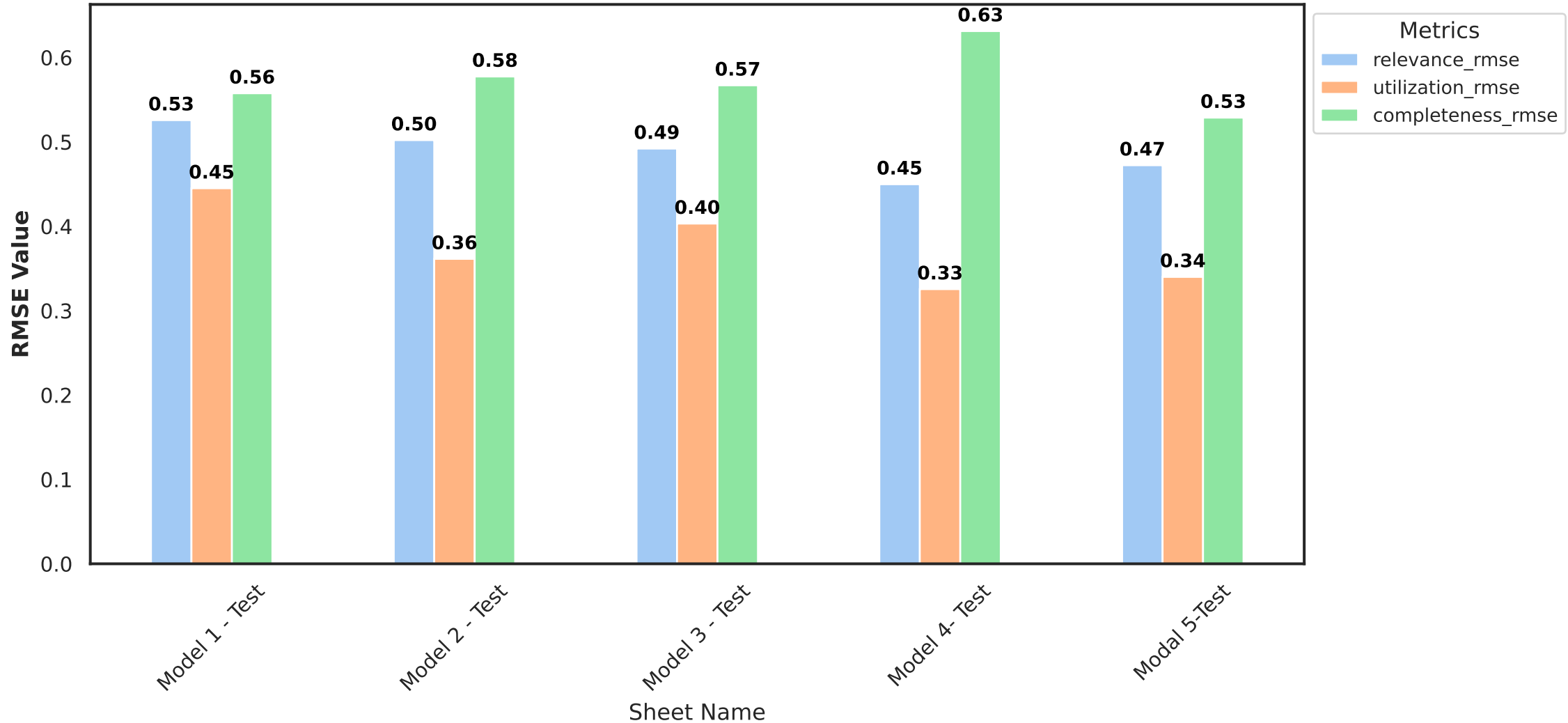
RMSE Comparison (Test Split)
